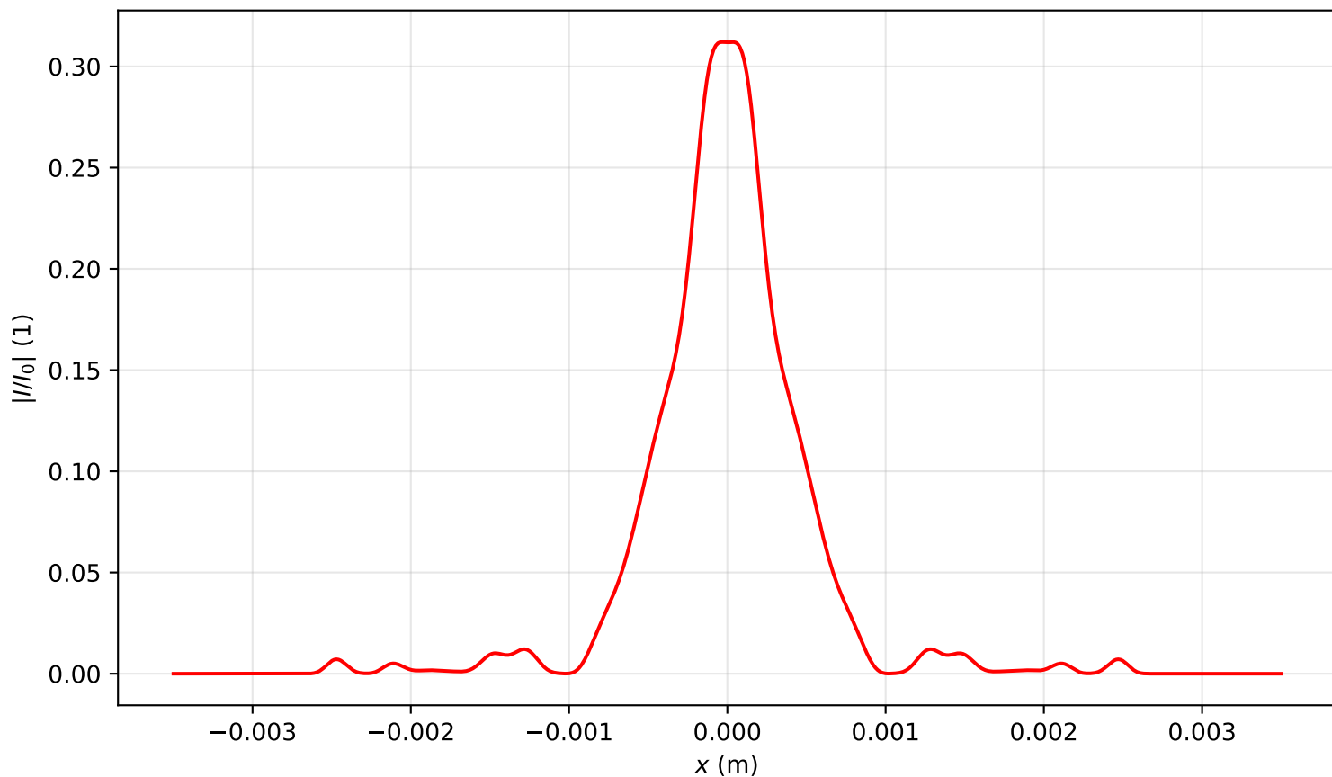
Intensity profile I(x, y = 0, z = 2.070)/I_0 , P_{in}=4.0P_{cr} , artificial time
